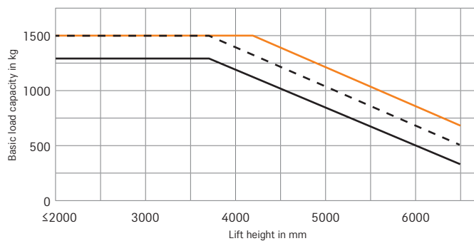
RCE 15 Triplex mast - superelastic tyres
