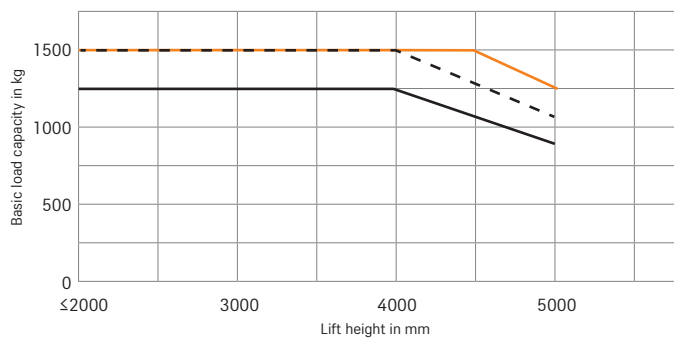
RCE 15 Telescopic/HiLo mast - superelastic tyres
